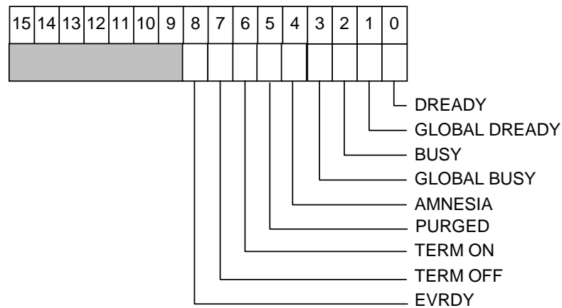
Fig. 4.16: Status Register 1
