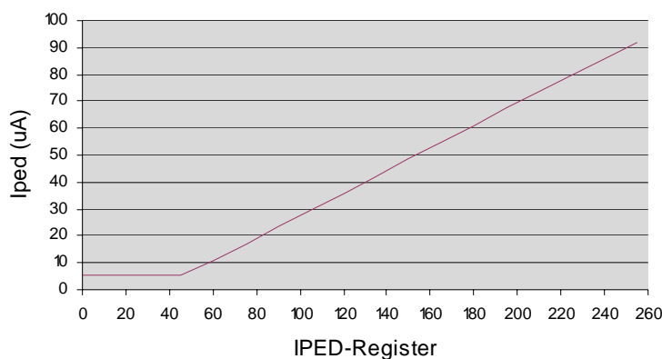
Fig. 2.6: Iped ( \mu A) Vs IPED-Register setting
